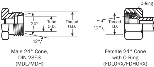
DIN 24° Male and Mating Females
