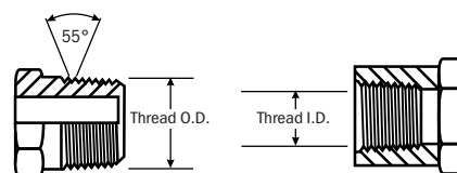
BSPT Male (MBSPT)
