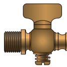
Air Shut-Off Cock - Male Pipe - Bibb Nose with Key Handle G33832
