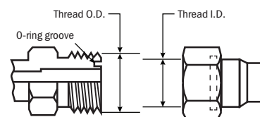
Male British Flat-Face (MBFF)
