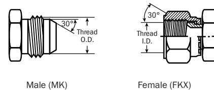
Komatsu Style 30° Flare
