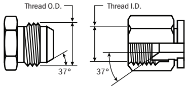
JIC 37° Male (MJ) JIC 37° Flare Female (FJX)
