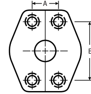
4-Bolt Split Flange Bolt Hose Dimensions
