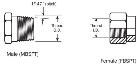
Japanese Tapered Pipe Thread
