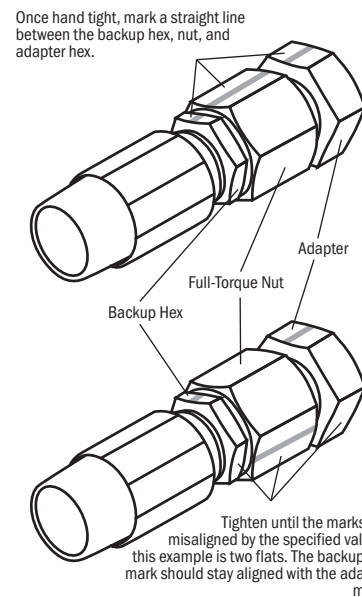
Figure 2 Flats method of verifying coupling torque.
