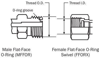
O-Ring Face Seal
