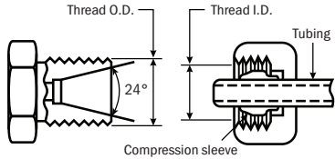
Male flareless assembly (MFA) includes sleeve (FFS) and nut (FFN)
