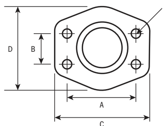
Flange Clamp
