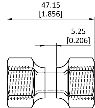
ASSEMBLY VIEW
